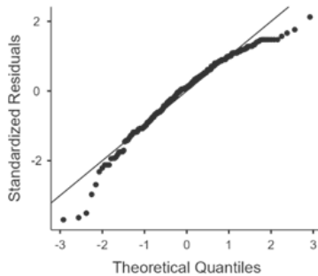
Figure 1: Normality Q-Q Plot of T-Test
