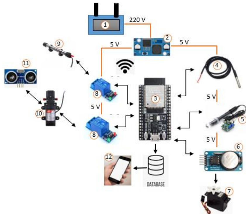
Fig.1. The complete system circuit
