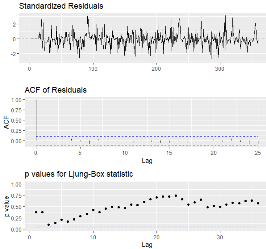
4 Gambar 6. Plot diagnostik Model ARIMA(1,1,1)(0,1,1)[12]
