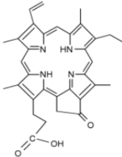
Gambar 9.1 Pyropheophorbide-A
