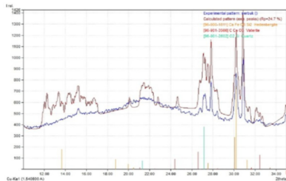
Figure 2. Analysis XRD for cacao shell charcoal
