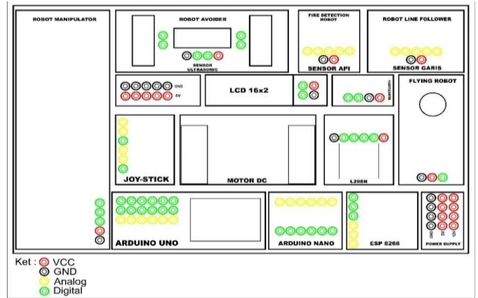
Figure 1. Layout of Robotics Trainer Media.
