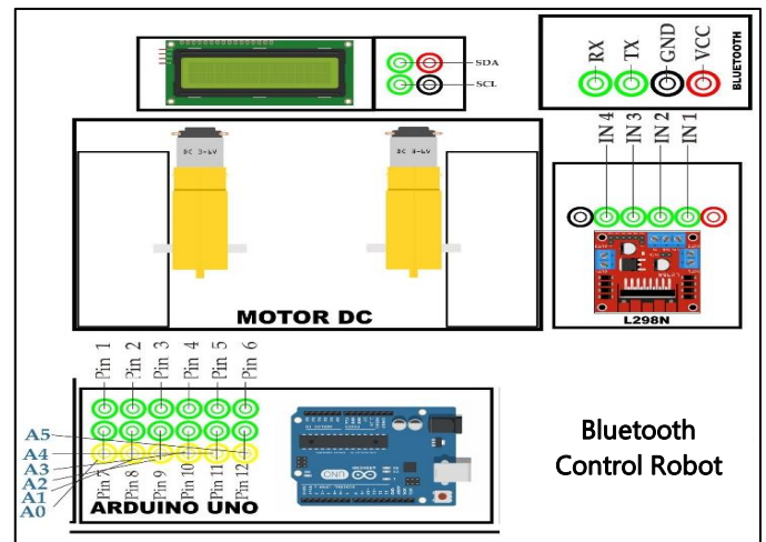
Figure 2. Robotics Trainer Media Circuit.
