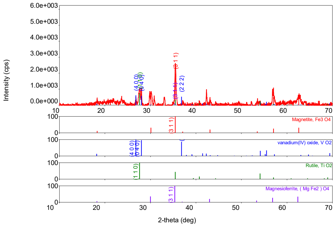
Figure 2. X-ray diffraction pattern of MA2 sample
