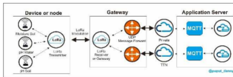
Fig. 2. LoRa Architecture
