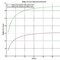
Fig. 6. Battery life (hours) of modification delay
