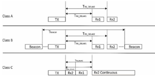
Fig. 3. LoRaWAN class
