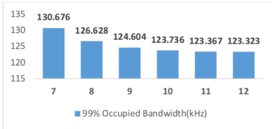
Fig. 17. 99% Occupied Bandwidth (kHz) and SF comparison
