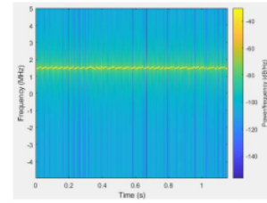
Fig. 14. Chirp signal LoRa 915 MHz Frequency analyzes SF12, 125 kHz, PTx 14 dBm
