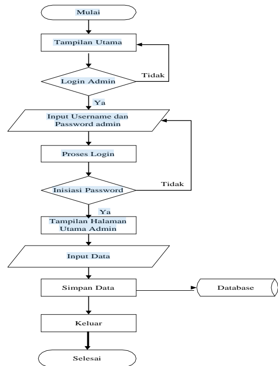
Gambar 1 Flowchart
