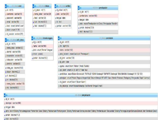
Gambar 3 Database
