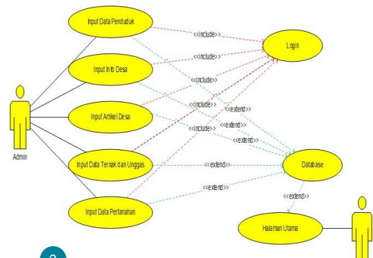
2 Gambar 2 Use Case Diagram
