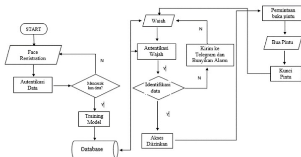
Gambar 7. Flowchart Sistem
