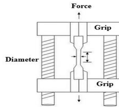
Gambar 3: Proses uji tarik
