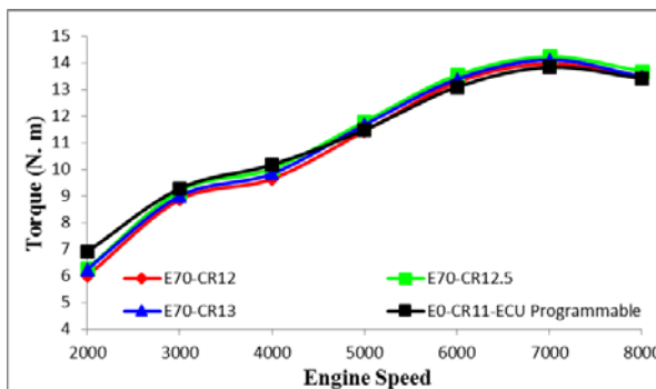
Figure 10. Graph of Torque Variation of Compression Ratio as Engine Speed Function
