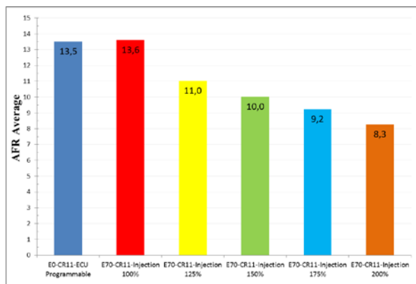
Figure 7. Graph Average AFR Variation Injection
