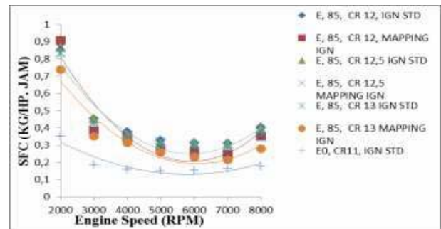
Figure 8. Specific Fuel Consumption Vs Engine Speed Specific fuel consumption E85 will be greater than that of
