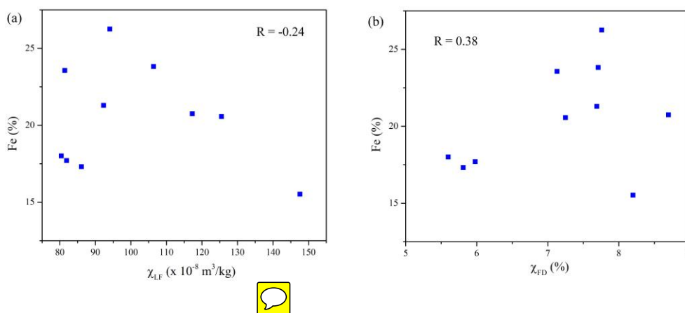
Figure 5. Plot of (a) \chi_{LF} with Fe and (b) \chi_{FD} with Fe.
