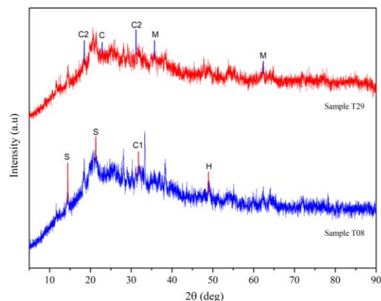
Figure 4. XRD diffractogram of extracted Bat Cave guano sample where S=silicon dioxide ( \text{SiO}_2 ), C1=calcium indium ( \text{Ca}_3\text{In} ), H=hexaferrum (Fe), C2=calcium aluminum antimonide ( \text{Ca}_{14}\text{AlSb}_{11} ), M=magnetite ( \text{Fe}_3\text{O}_4 ), C=calcium aluminum antimonide ( \text{Ca}_{14}\text{AlSb}_{11} ).
