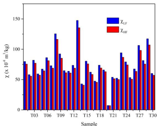
Figure 2. Histogram of magnetic susceptibility at low ( \chi_{\text{LF}} ) and high frequency ( \chi_{\text{HF}} ) of Bat Cave guano samples.
