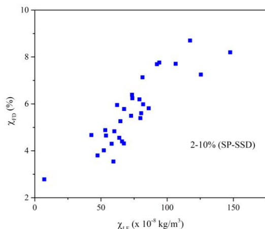
Figure 3. Scattering of frequency-dependent ( \chi_{\text{FD}} ) and low-frequency ( \chi_{\text{LF}} ) magnetic susceptibility of Bat Cave guano samples.
