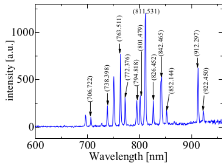
Figure 3. The emission line spectrum of Argon I from argon plasma jet under atmospheric pressure
