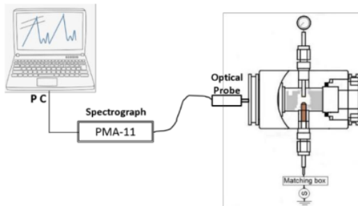
Figure 2. Multichannel spectral analyzer
