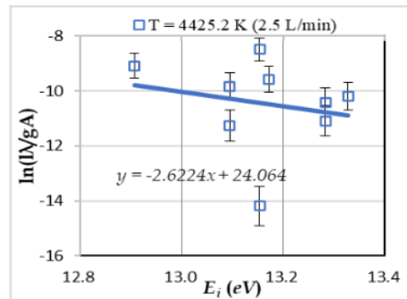
Figure 9. Excitation temperature at 2.5 L/min
