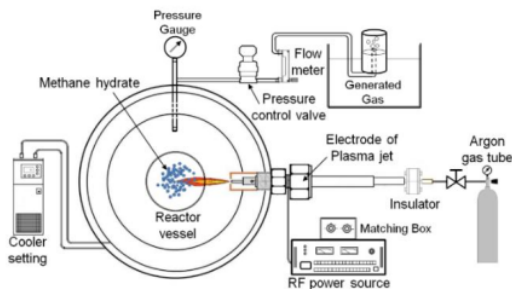
Figure 1. High-frequency argon jet plasma mechanism
