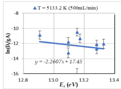
Figure 6. Excitation temperature at 500mL/min
