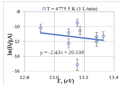
Figure 7. Excitation temperature at 1 L/min
