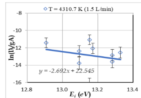
Figure 8. Excitation temperature at 1.5 L/min
