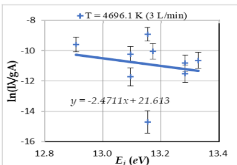
Figure 10. Excitation temperature at 3 L/min
