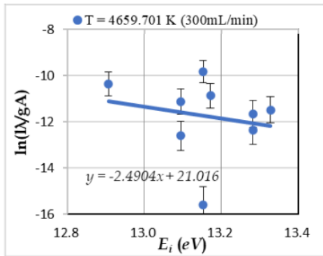
Figure 4. Excitation temperature at 300mL/min
