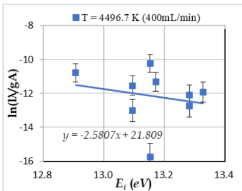
Figure 5. Excitation temperature at 400mL/min
