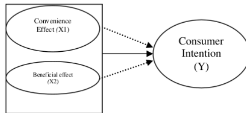
Figure 1. Research Framework
