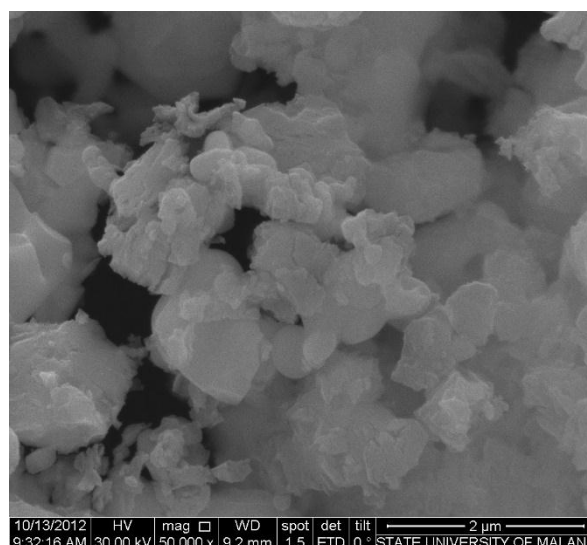
Figure 3. Morphology of \text{Nd}_{1.2}\text{FeO}_3 sample at a higher magnification
