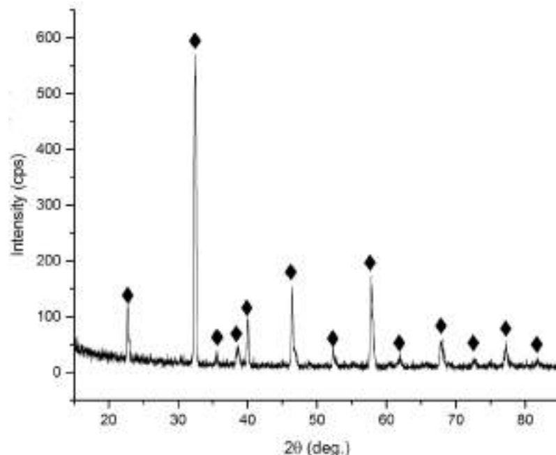
Fig. 1 XRD pattern of \text{Nd}(\text{Fe})\text{BaCuO} ( \blacklozenge = \text{Nd}(\text{Fe})\text{BaCuO} ).
