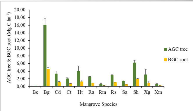
Figure 4. AGC and BGC stocks of mangrove species include the standard error of the mean.
