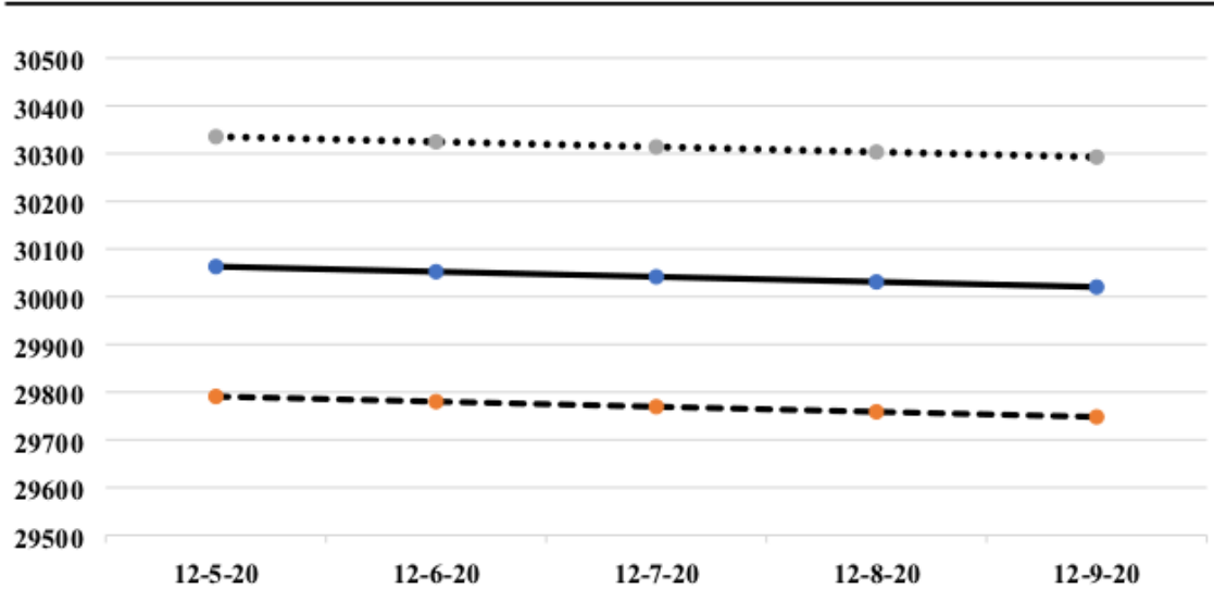
Fig.4 Forecast for Closing Stock Price DJI in the USA (with 99% Upper & Lower Limit)
