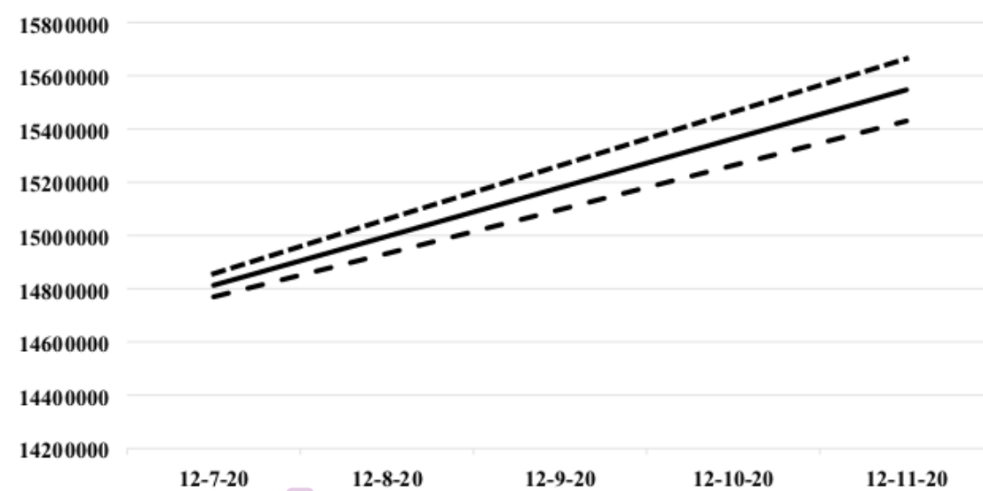
9 Fig. 3 Forecast for confirmed cases of COVID-19 in the USA (with 99% Upper and Lower Limit)
