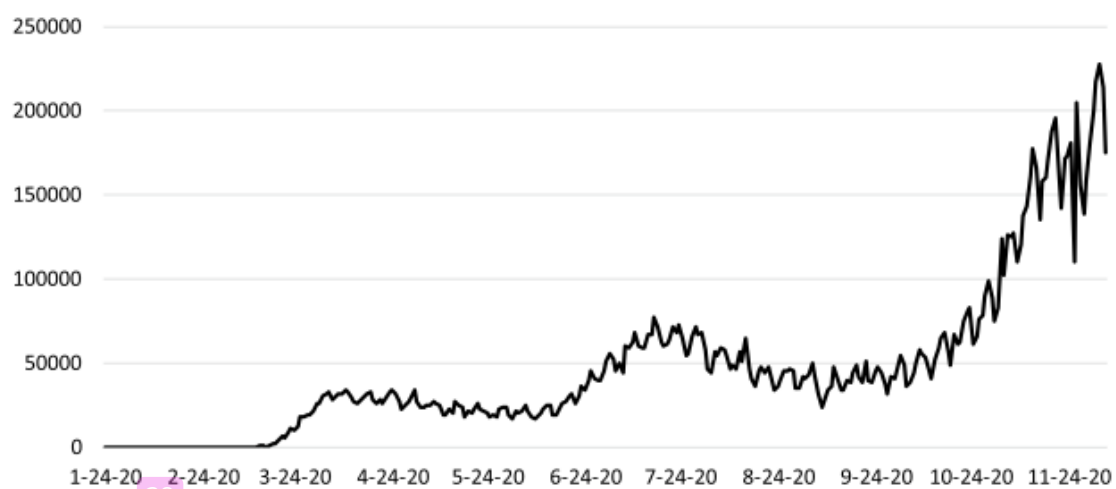
38 Fig. 1 Daily New Cases of COVID-19 in the USA
