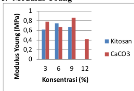
Gambar 6. Perhitungan Modulus Young
