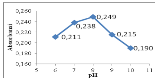
Figure 3. Calibration curve of absorbances for pH optimum of EDTA.
