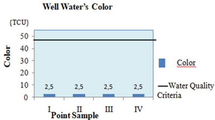
Figure 2. Histogram of Well Water's Color RT 04 RW 11 Parang Tambung Sub-District Tamalate District Makassar City Tahun 2017. The results obtained in the color of well water samples at all locations are 2.5 units PtCo/color.
