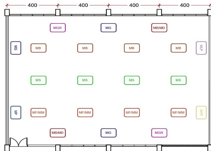
Fig. 1. Layout Laboratory Tooling Machine Unit (Research Location).
