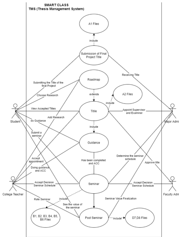
Fig 4. Use Case diagram of Thesis Management System
