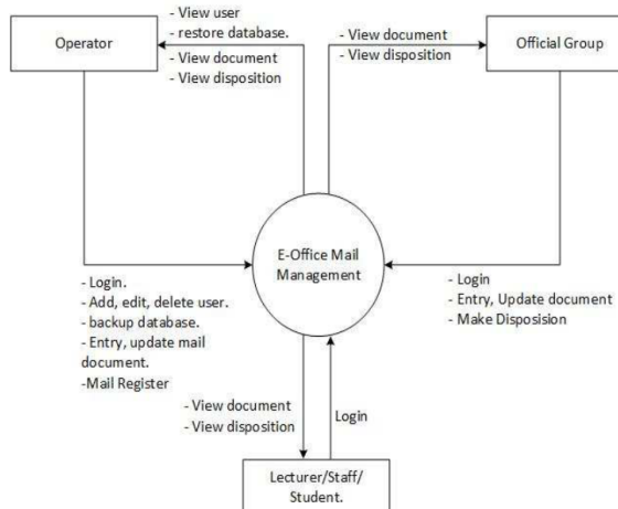
Fig 6. College E-Office System Context Diagram
