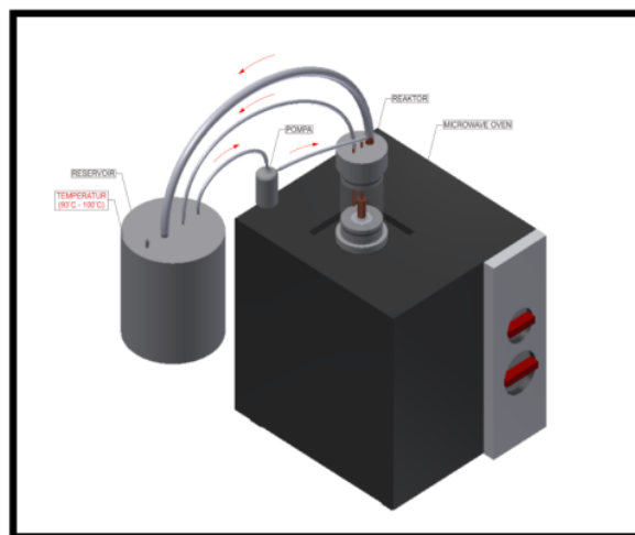
Fig.1 Experimental Apparatus
