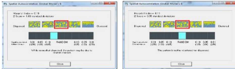
Figure 2: Results of Global Moran's I for dengue cases in January and December in 2013 using ArcGis
