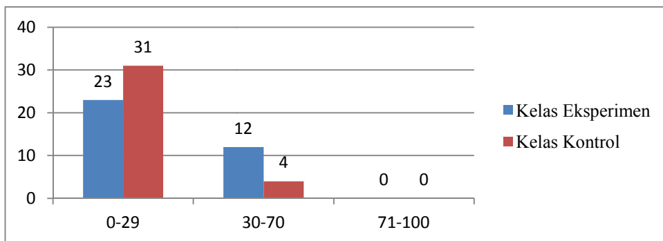
Gambar 2. Diagram N-Gain siswa
