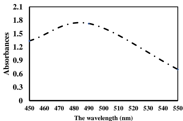
Figure 1. The wavelength optimization of DCR dyestuff
