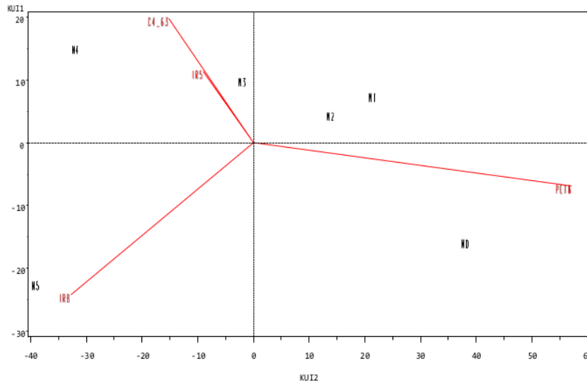
Figure 1. Biplot of AMMI-2 Model
