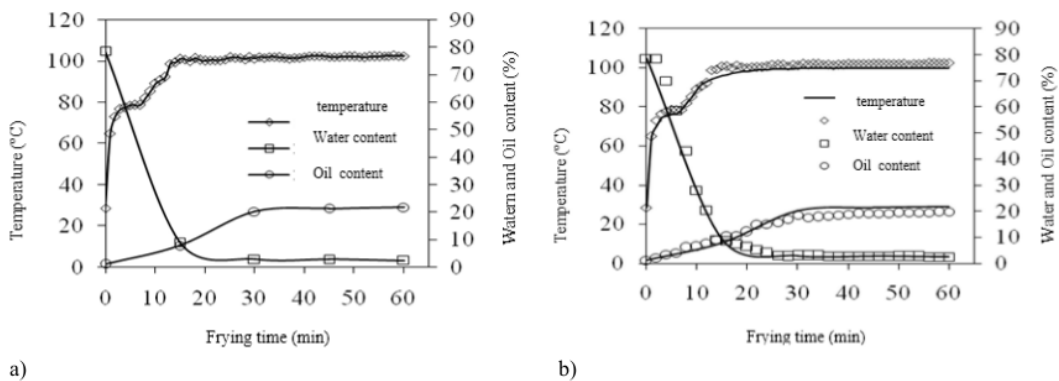
Figure 5: History temperature, moisture reduction and oil absorption simultaneously in jackfruit solids during the frying process at the oil temperature of 100°C with the vacuum pressure of 90 kPa; a) observational data; and b) the results of simulation models.
