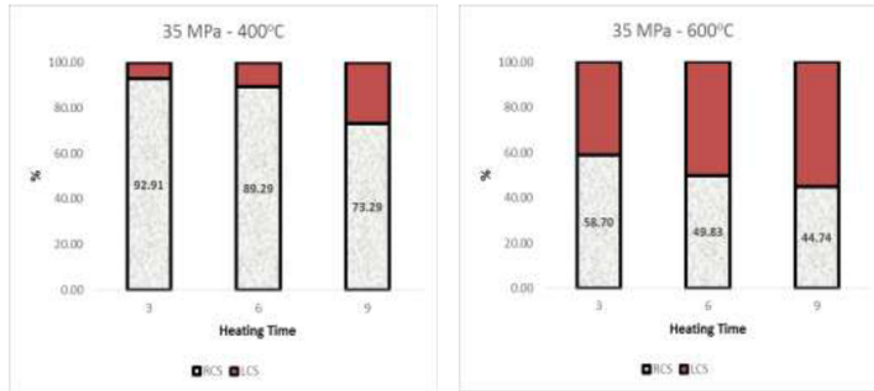
15 Fig.6. Residual Strength of Concrete (TS 35)
