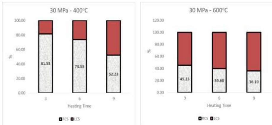
6 Fig.5. Residual Strength of Concrete (TS 30)
