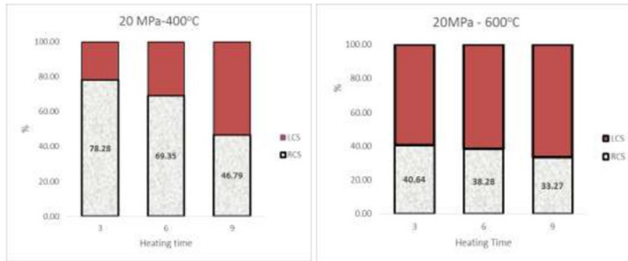
6 Fig.4. Residual Strength of Concrete (TS 20)
