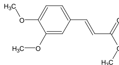
(i) 3-[3,4-dimethoxyphenyl]-methyl ester
