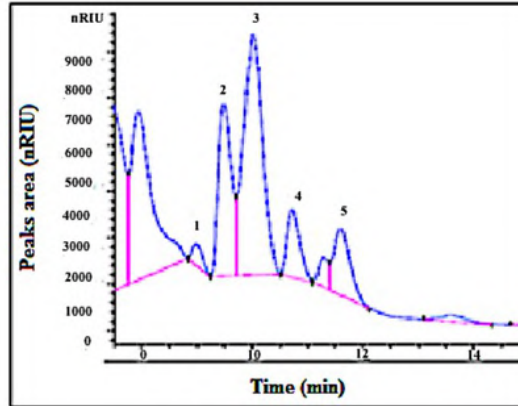
FIGURE 1. Monosaccharide content contained in pectin from Nephrolepis biserrata leaves (1) Xylose, (2) Rannose, (3) Arabinose, (4) Mannose, (5) Galactose.
