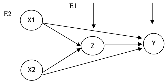
Gambar 3.2 Diagram model path analisis penelitian
