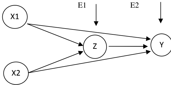
Gambar 4.5 Diagram model path analisis penelitian
